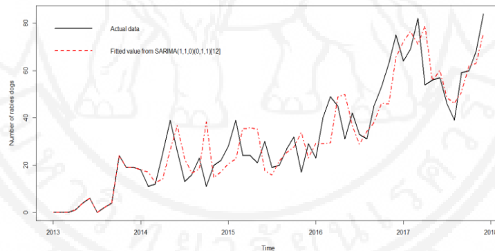
Figure 4 Comparison of the actual number of rabies in dogs with fitted values from the SARIMA model in Thailand 2013 to 2017
