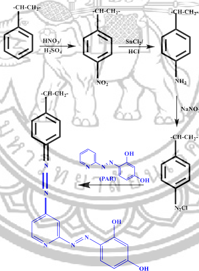
Figure 1 The methodology of the modified Amberlite XAD-4/PAR resin.
