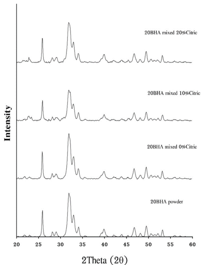
Figure 6 XRD patterns of the 20BHA with different concentration of citric acid after 21 days of setting.
